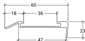
AD GLO 60mm stair tread nosing cross section
