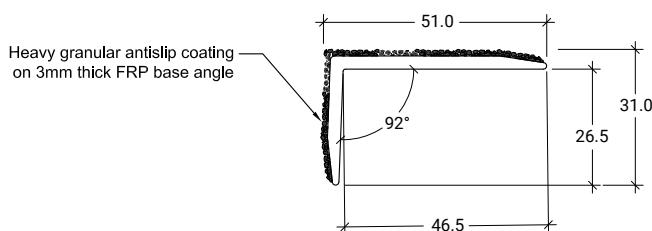
MFRP 50mm profile cross section
