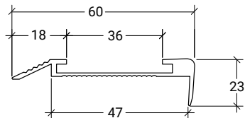
AD 60mm stair tread nosing cross section
